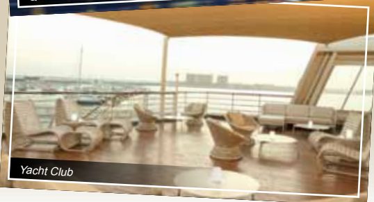
Queen Elizabeth 2
